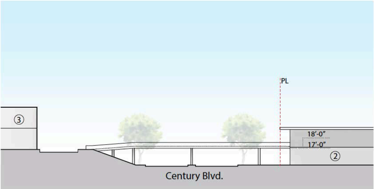
Figure 2.7 Pedestrian Bridges
