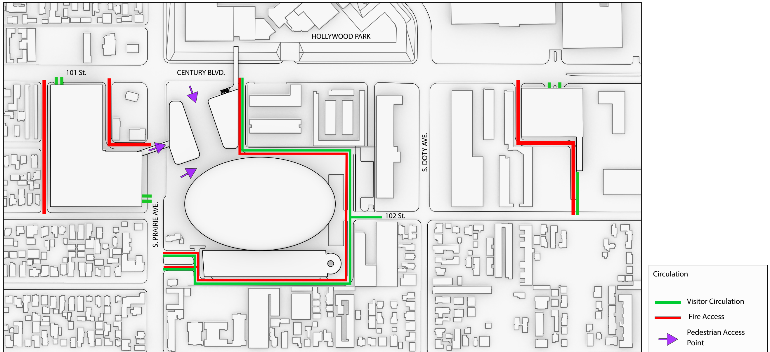
Figure 6.1 Circulation
