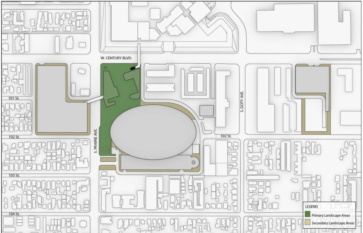
Figure 3.1 Landscape Design Areas
