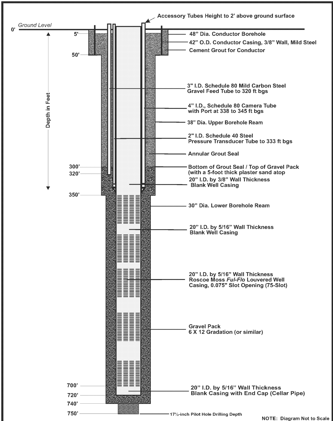
FIGURE 8 PRELIMINARY WELL DESIGN DIAGRAM PROPOSED WELL NO. 8
