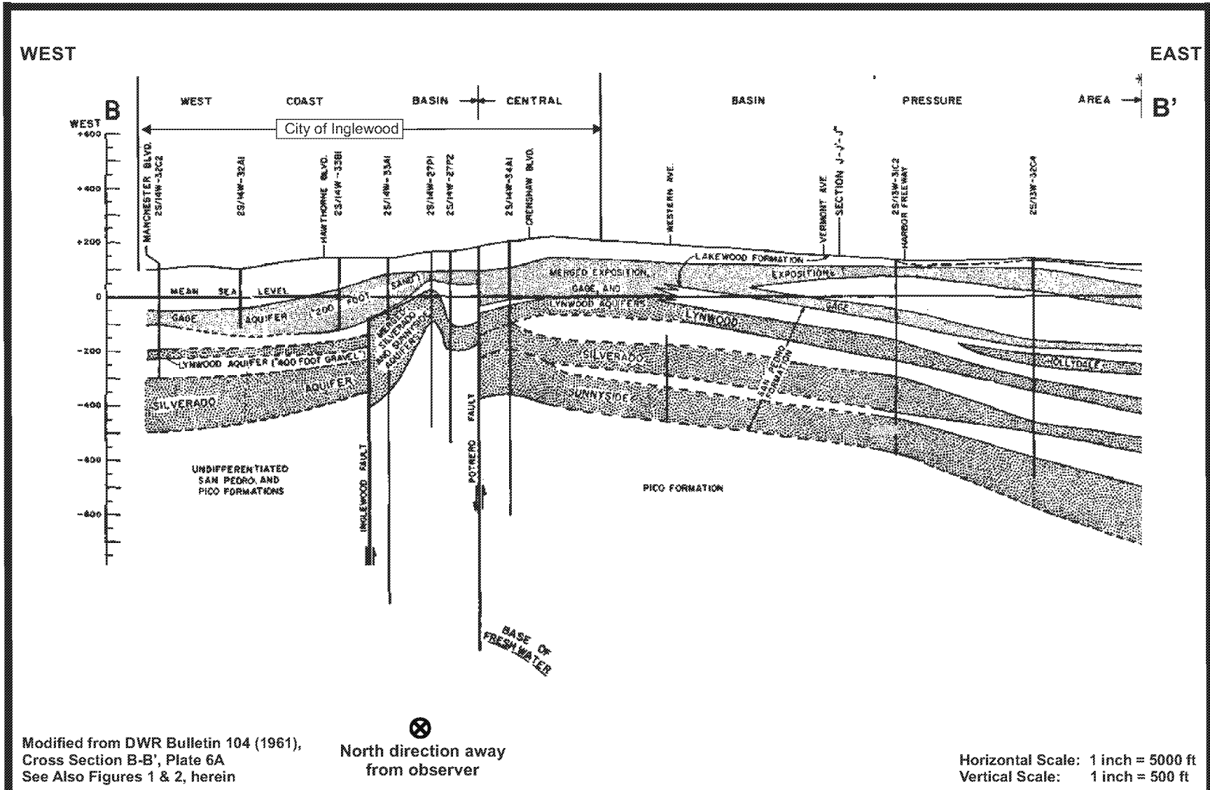
FIGURE 3 GENERALIZED GEOLOGIC CROSS SECTION B-B' CITY OF INGLEWOOD REGION
