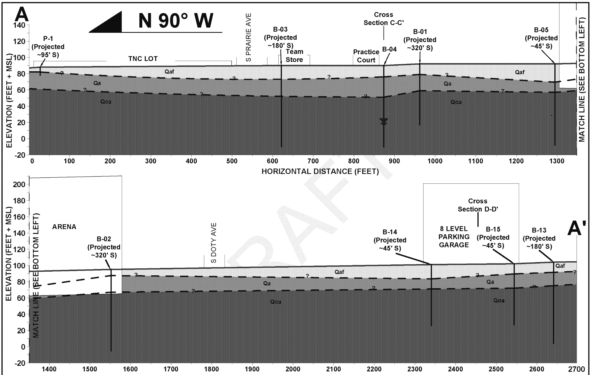
CROSS SECTION A-A' PROJECT CONDOR SE CORNER OF PRAIRIE AVENUE & W. CENTURY BOULEVARD INGLEWOOD, CALIFORNIA FOR: MURPHY'S BOWL, LLC
