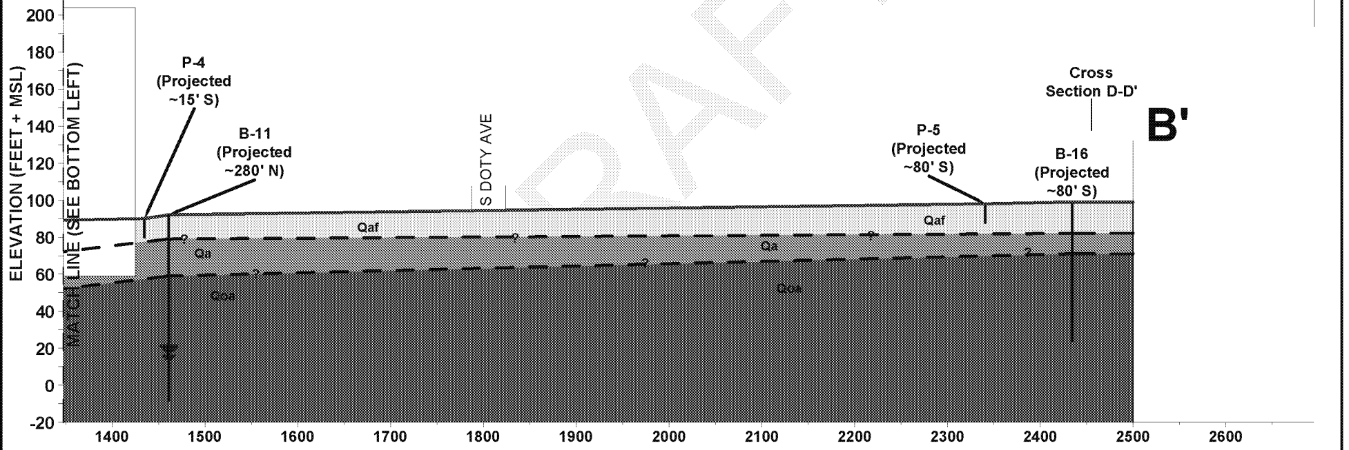
CROSS SECTION B-B' PROJECT CONDOR SE CORNER OF PRAIRIE AVENUE & W. CENTURY BOULEVARD INGLEWOOD, CALIFORNIA FOR: MURPHY'S BOWL, LLC
