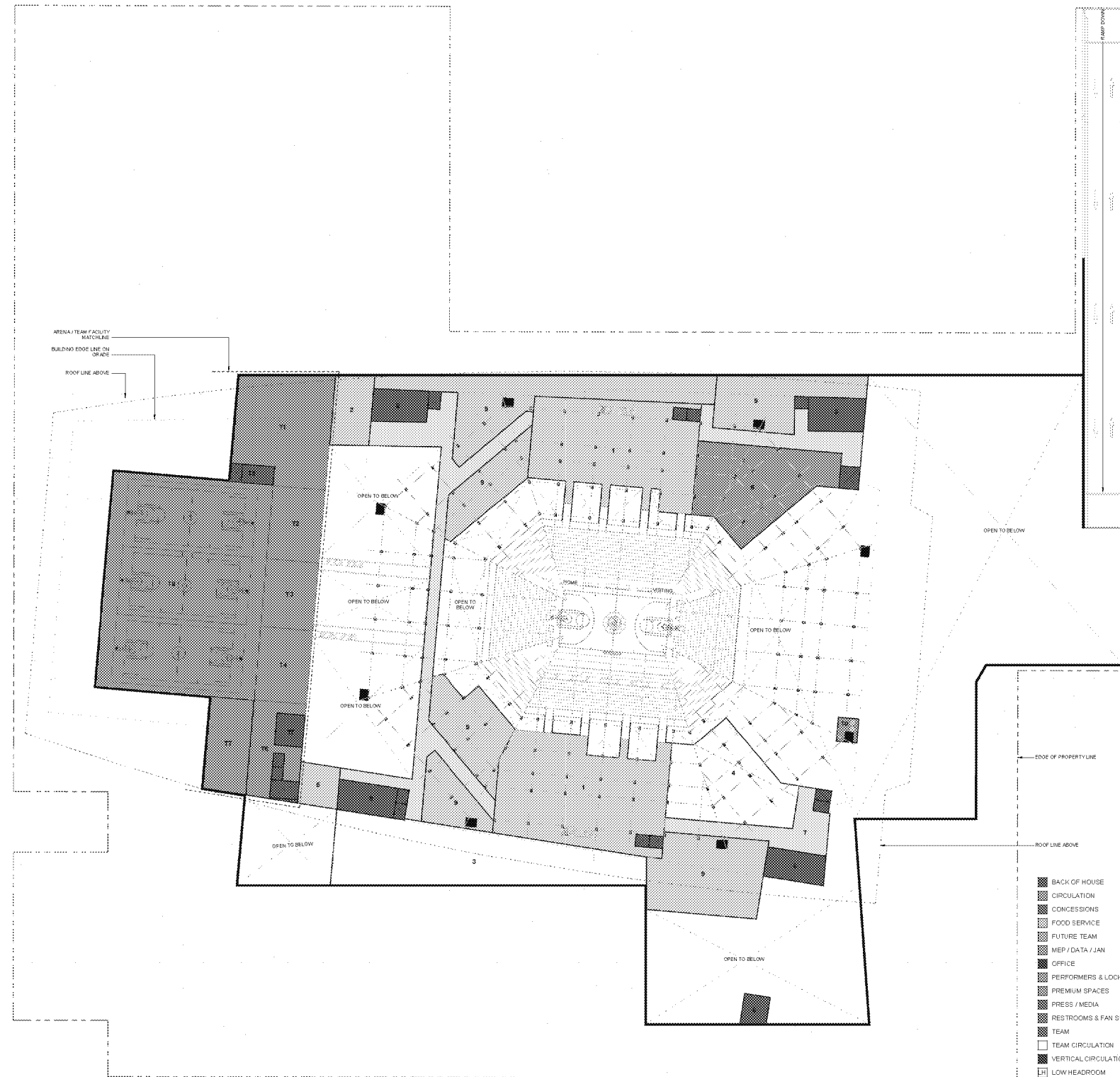
1 CLUB LEVEL FLOOR PLAN 1/32" = 1'-0"
