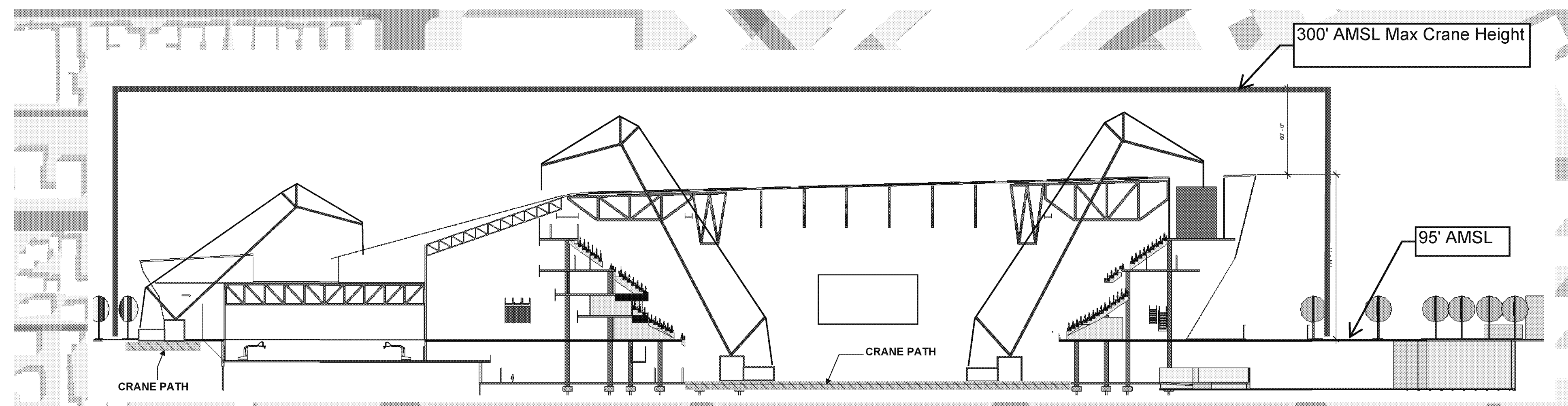
SECTION - A
