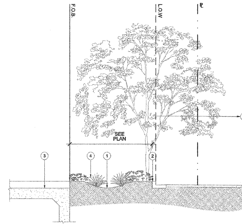
3 LANDSCAPE SECTION SCALE: 1/4"=1'-0" 0 4 8 12
