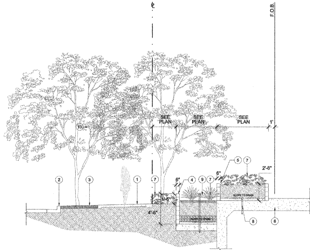
5 LANDSCAPE SECTION SCALE: 1/4"=1'-0" 0 4 8 12
