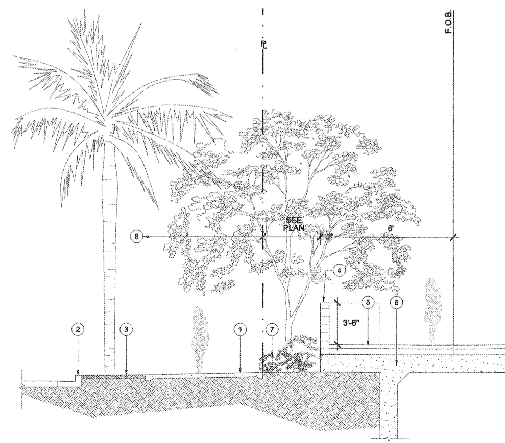
1 LANDSCAPE SECTION SCALE: 1/4"=1'-0" 0 4 8 12
