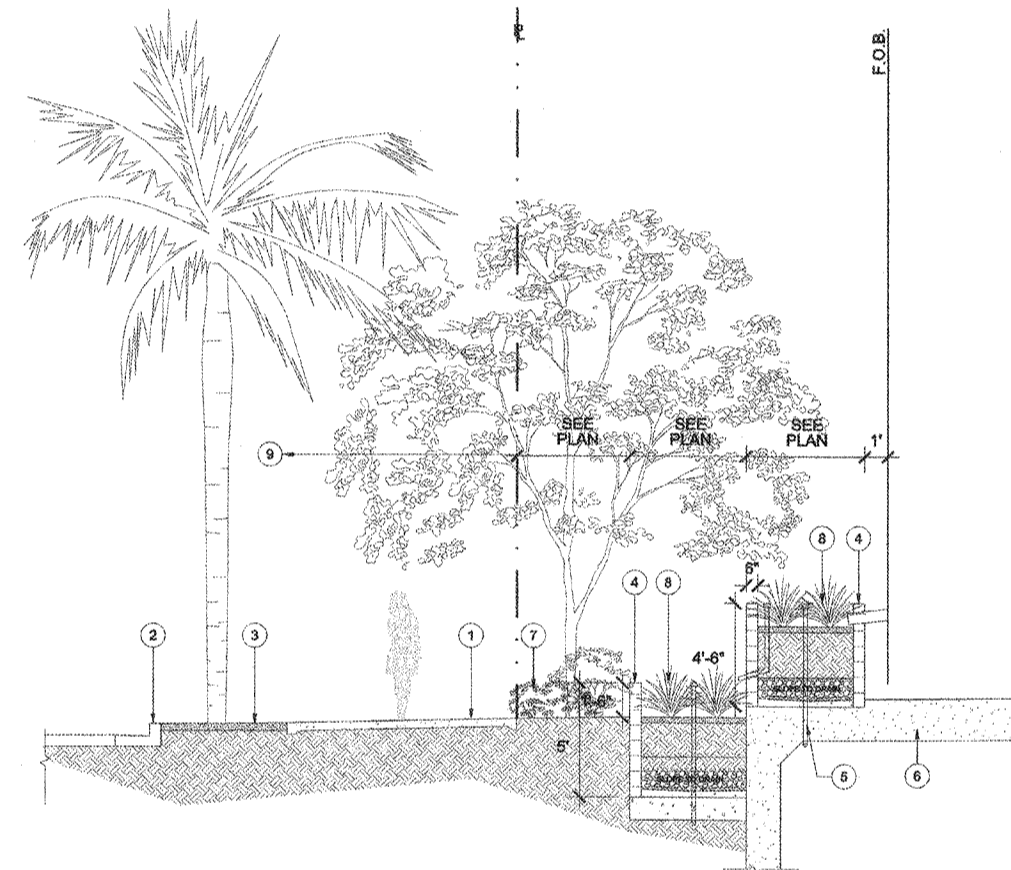
2 LANDSCAPE SECTION SCALE: 1/4"=1'-0" 0 4 8 12
