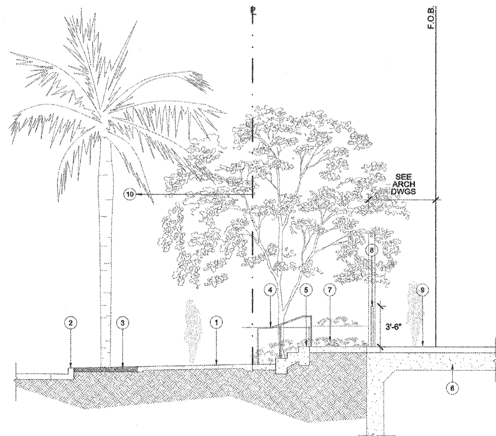
4 LANDSCAPE SECTION SCALE: 1/4"=1'-0" 0 4 8 12
