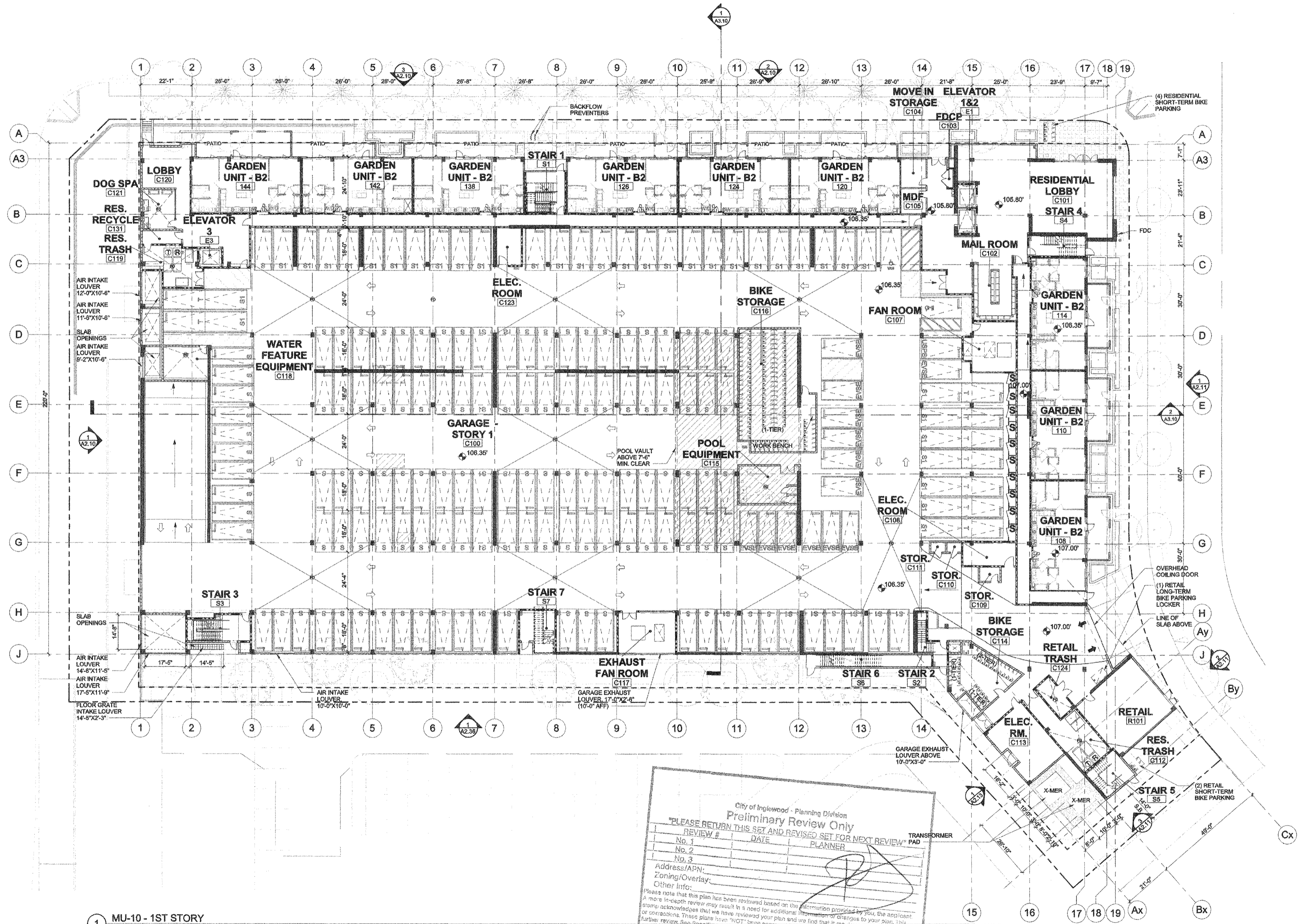
1 MU-10 - 1ST STORY 1/16" = 1'-0" 0 16 32 64
