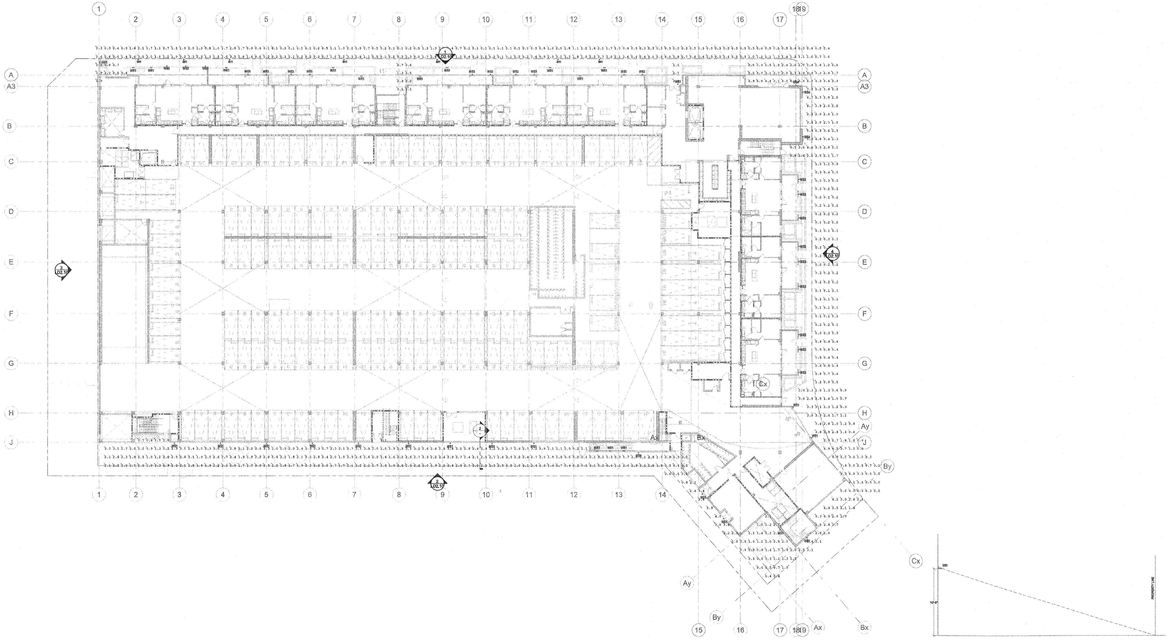
1 1ST STORY 1/16" = 1'-0" 0 16 32 64
