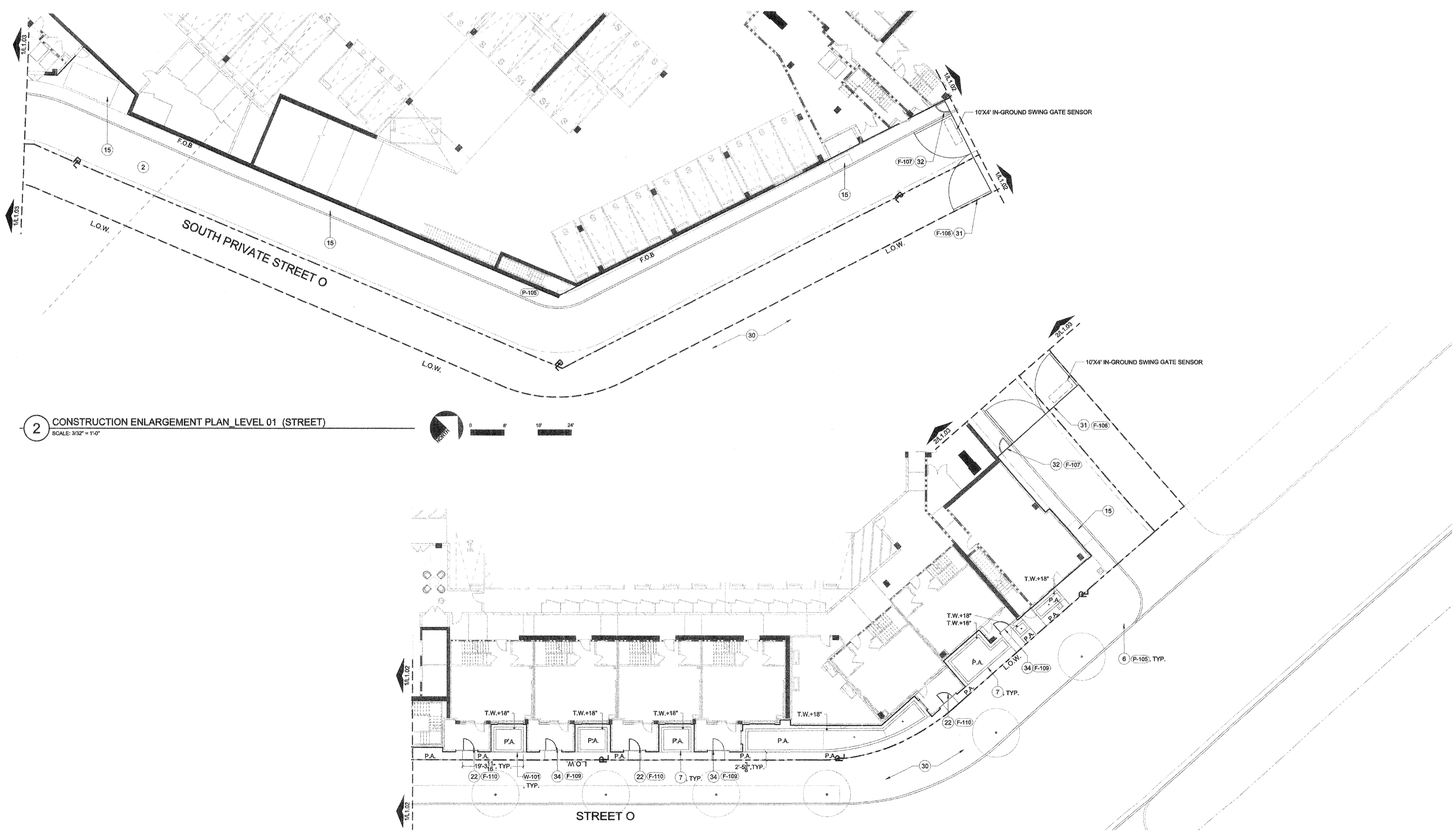
1 CONSTRUCTION ENLARGEMENT PLAN_LEVEL 01 (STREET) SCALE: 3/32" = 1'-0"
