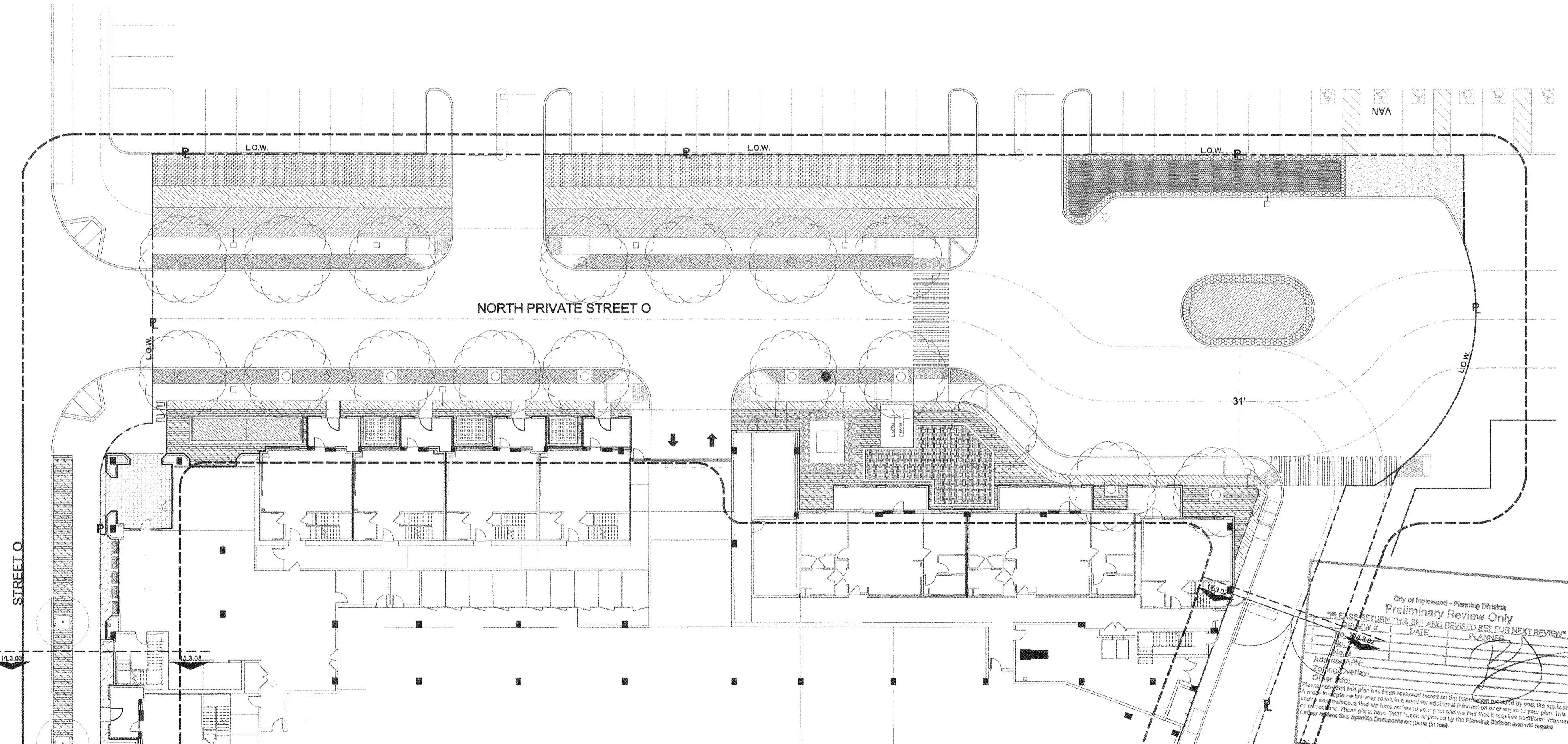
1 LANDSCAPE PLANTING PLAN LEVEL 1 ENLARGEMENT SCALE: 3/32" = 1'-0"
