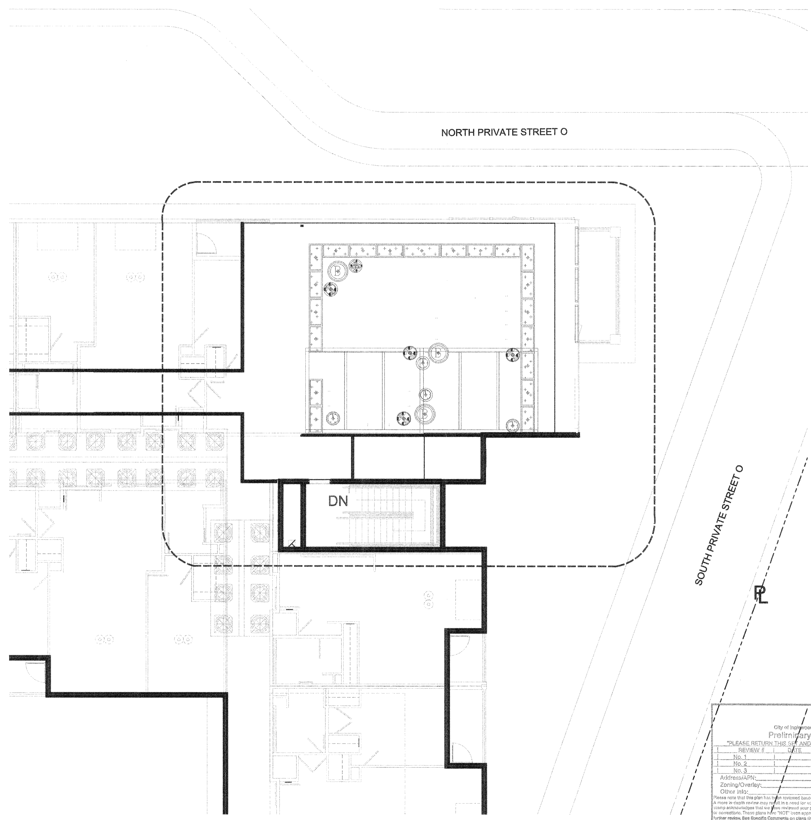
1 LANDSCAPE PLANTING PLAN LEVEL 06 (ROOF) ENLARGEMENT SCALE: 1/4" = 1'-0"
