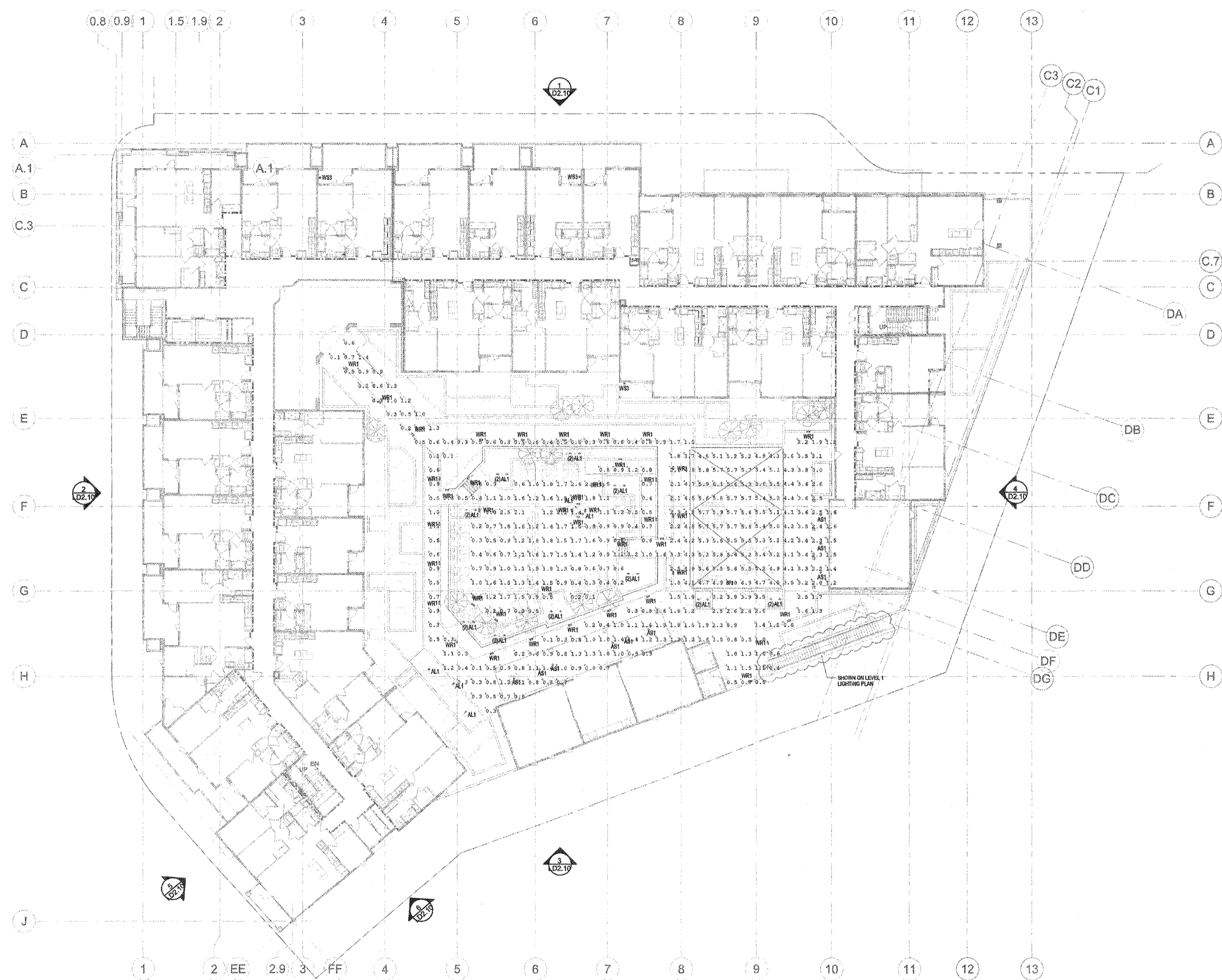
1 3RD STORY 1/16" = 1'-0" 0 16 32 64
