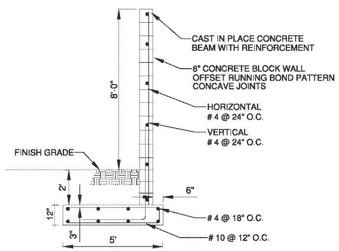
SECTION A-A 1" = 2'-0"
