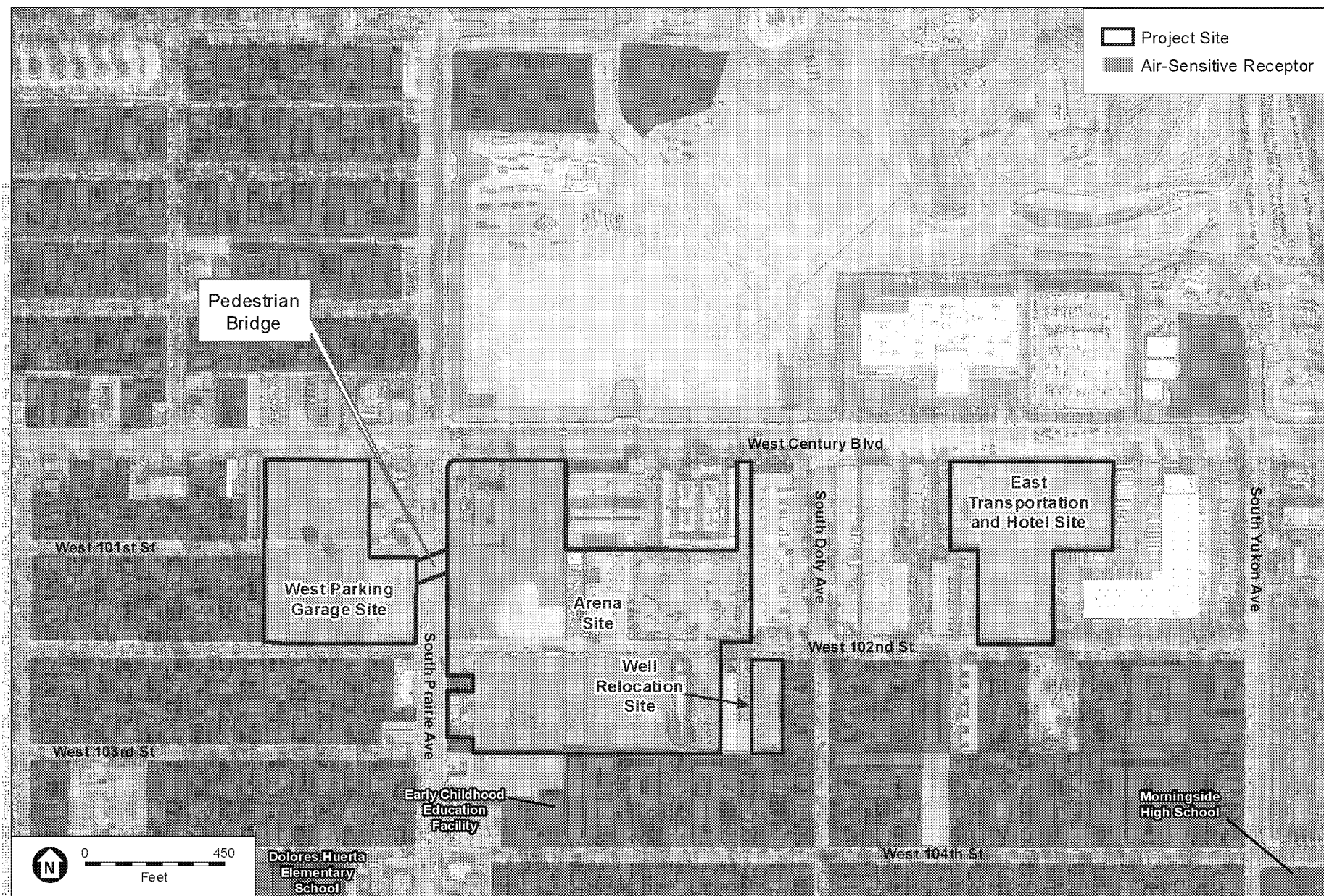
Figure 3.2-2 Air-Sensitive Receptors
